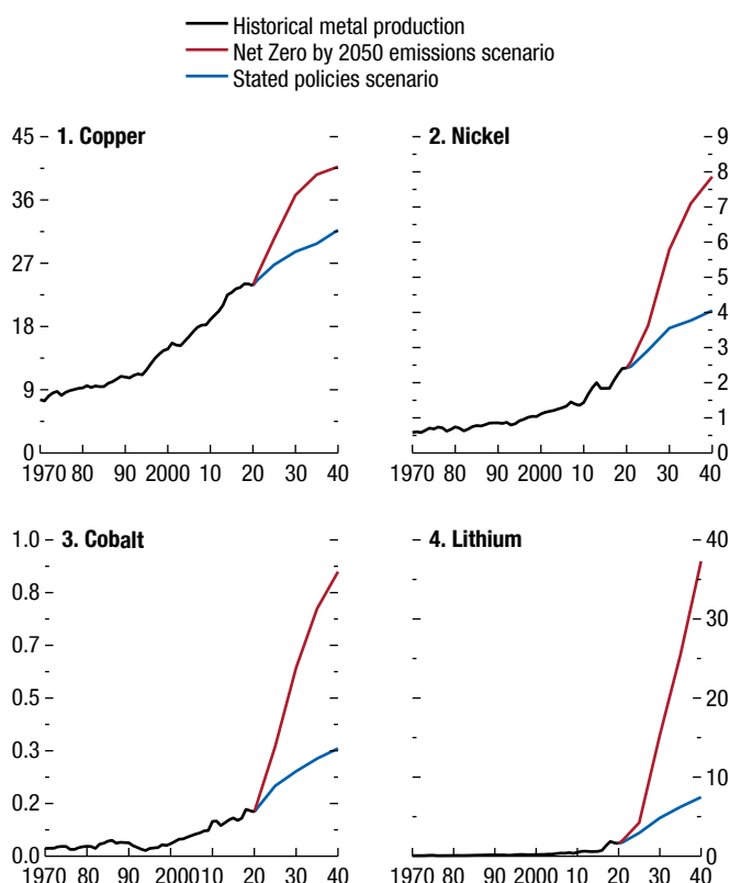
Figure 1.SF.4. Historical Metal Production and IEA Energy Transition Scenarios
