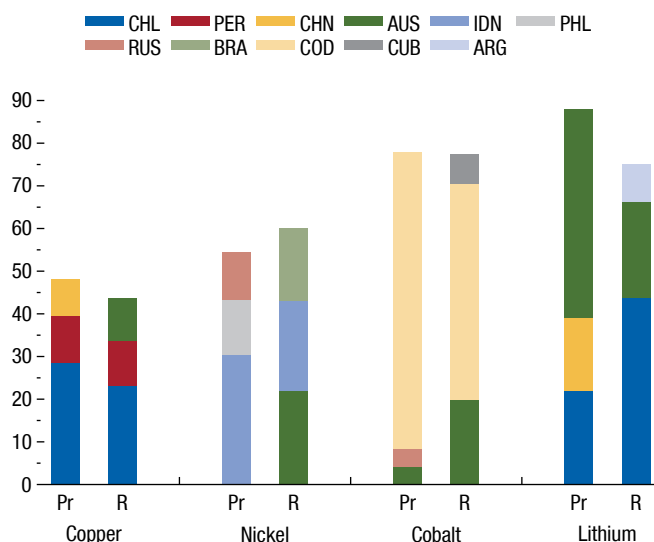
Figure 1.SF.5. Top Three Countries, by Share of Global Production and Reserves for Selected Metals
